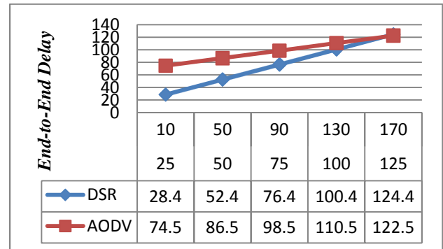
Figure (ii): For 10 nodes of DSR and AODV Figure 2 (i) and (ii): End-to-End Delay vs. Time
