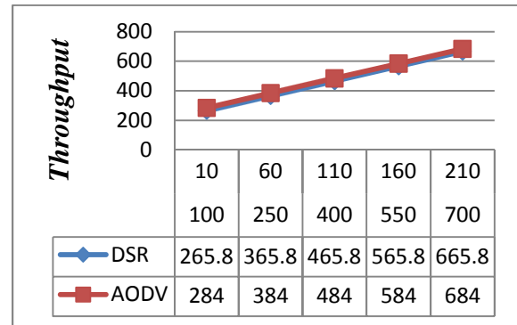
Figure (i): For 10 nodes of DSR and AODV Figure 4 (i) and (ii): Throughput vs Time
